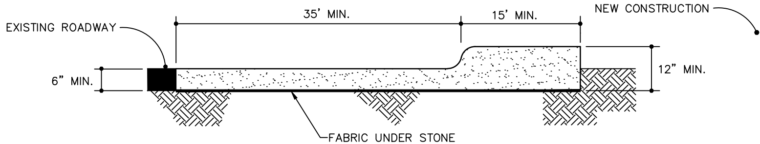
CROSS SECTION
