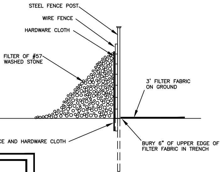
SECTION VIEW
